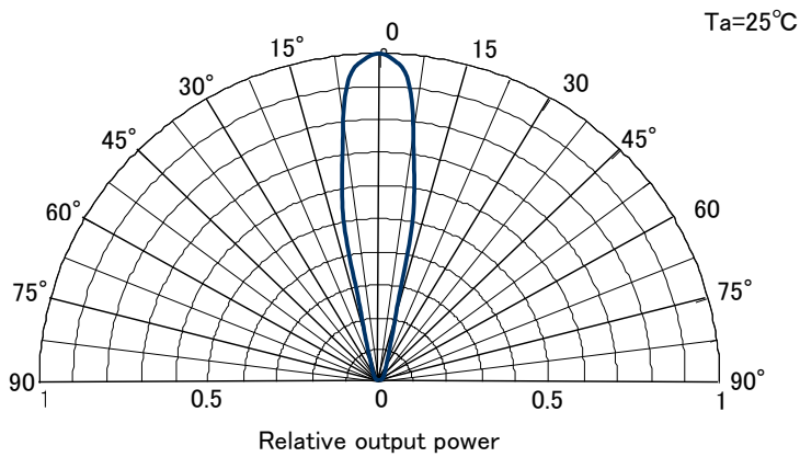
■ Directivity
